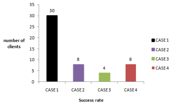
Fig 6 Success Rate
